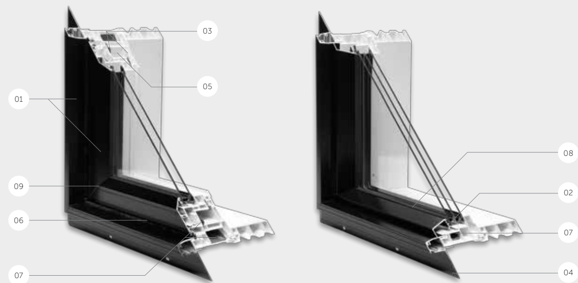
LynX Series Hybrid Casement & Awning Window Dual Glaze
