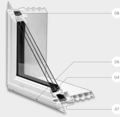
PVC Picture Window Triple Glaze
