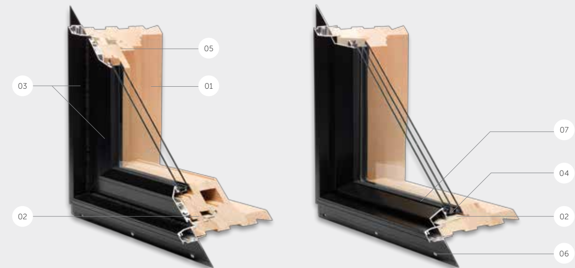
Aluminum Clad Casement & Awning Window Dual Glazed
